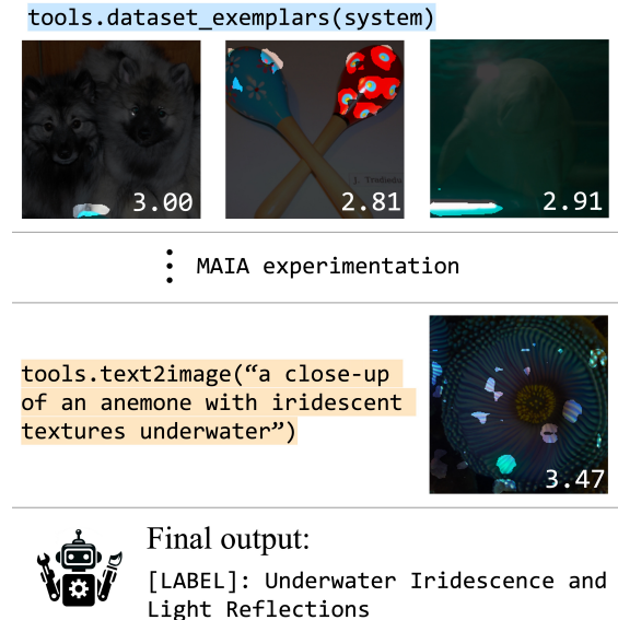
Figure A3. Example of MAIA having confirmation bias towards a single generated example, instead of generating further experiments to test other possibilities.
