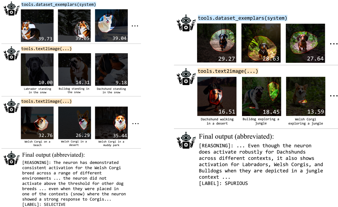
Figure A4. Two different MAIA interactions, classifying neurons as selective (L) and spurious (R).
