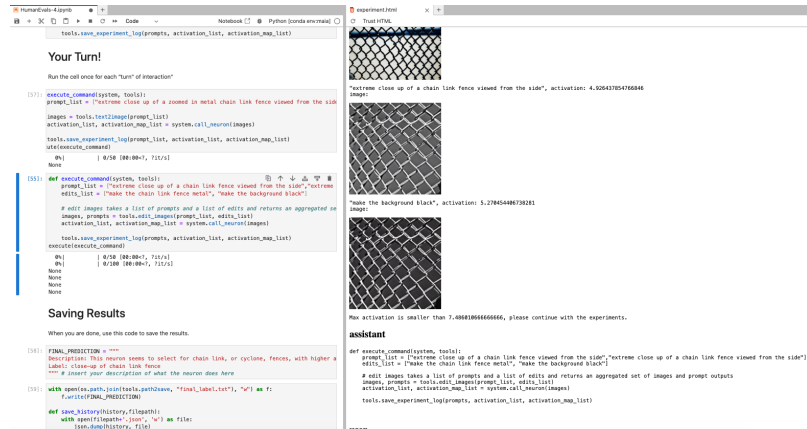
Figure A1. Example interface for humans interpreting neurons with the same tool library used by MAIA.
