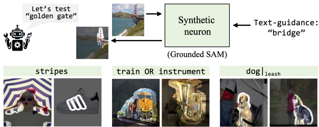
Figure 5. Synthetic neuron implementation. Segmentation of input images is performed by an open-set concept detector with text guidance specifying ground-truth neuron selectivity. Synthetic neurons return masked images and synthetic activation values corresponding to the probability a concept is present in the image.
