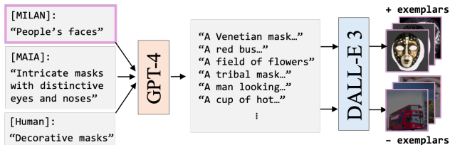
Figure 3. Generating predictive exemplar sets for evaluation.
