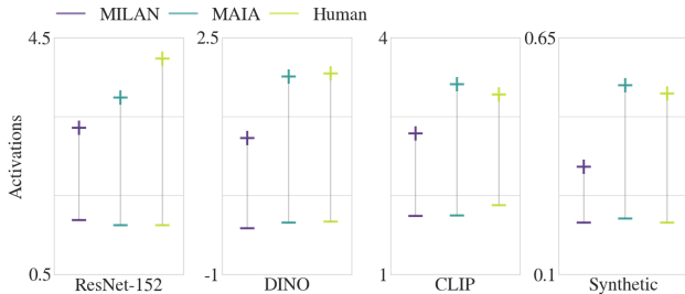
Figure 4. Predictive Evaluation. The average activation values for MAIA descriptions outperform MILAN and are comparable to human descriptions for both real and synthetic neurons.
