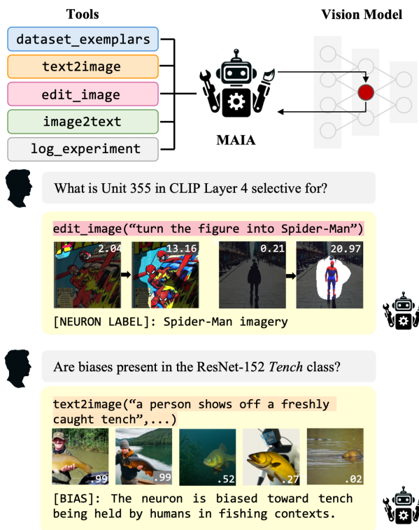
Figure 1. MAIA framework. MAIA autonomously conducts experiments on other systems to explain their behavior.
